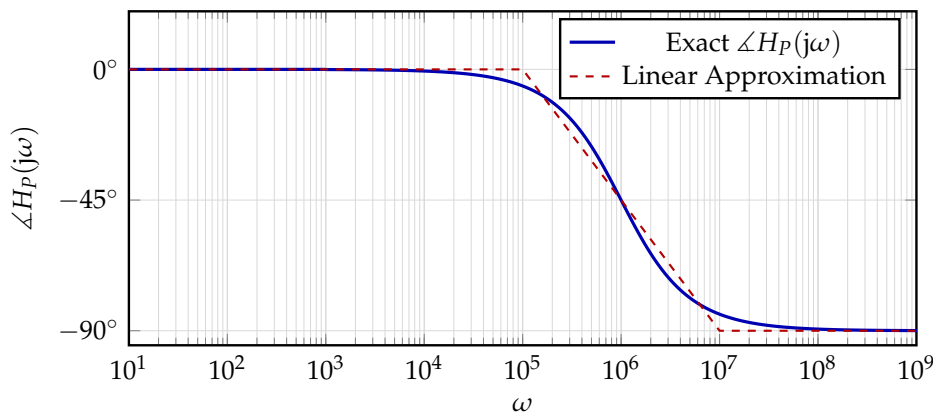
Figure 8: Simple Pole, Phase Plot.
